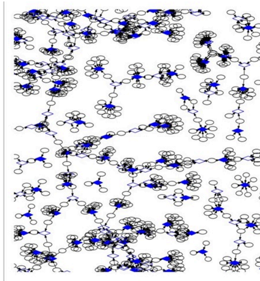
Figure 1. Left: Track-multiplicity dependence of the two-dimensional pion radius parameters obtained from fits for all collision systems studied. Lines are drawn to guide the eye.. Right: A small fraction of the bipartite graph of hits (ellipses) and track candidates (diamonds) for an event with multiple (40) pp collisions. Directed arrows, graph edges, show potential hit-to-track candidate assignments.
