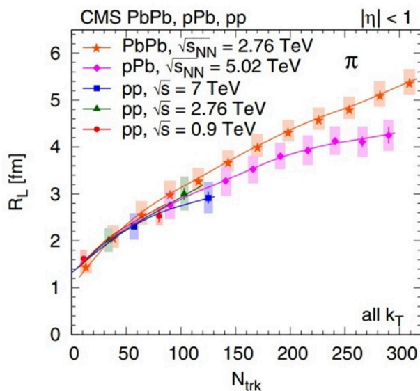
Figure 1. Left: Track-multiplicity dependence of the two-dimensional pion radius parameters obtained from fits for all collision systems studied. Lines are drawn to guide the eye.. Right: A small fraction of the bipartite graph of hits (ellipses) and track candidates (diamonds) for an event with multiple (40) pp collisions. Directed arrows, graph edges, show potential hit-to-track candidate assignments.
