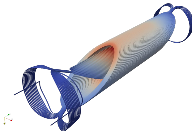
Figure 2. Winding geometry of the HTS CCT prototype
