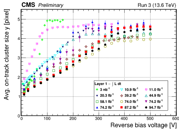
Figure 1. Change of cluster length as function of the bias voltage in the first part of 2024 data-taking. The plot demonstrates loss of charge collection efficiency and cluster breakage in the form of shorter average cluster length even at the operational bias voltage of 500 V [1].
