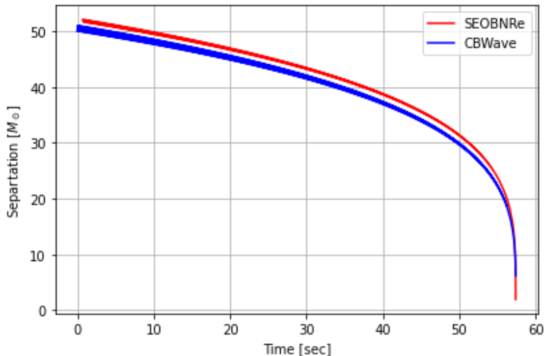
Caption: Radial dependence of SEOBNRe and CBWave frameworks.
