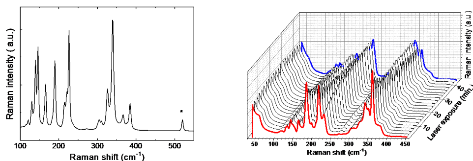
Figure 3. Raman spectrum of \text{As}_4\text{S}_5 crystallites prepared with nano-gold catalyst (left). In-situ photostructural transformation (realgar-pararealgar transition) of \text{As}_4\text{S}_4 (realgar type) crystallites prepared with nano-gold catalyst, measured by Raman spectroscopy (right).
