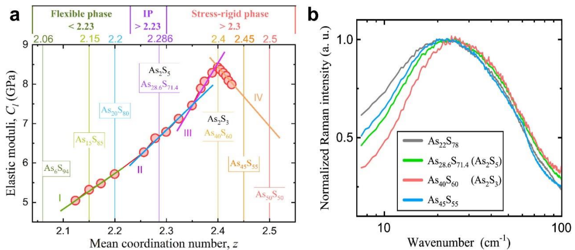
Figure 1. (a) Mean coordination number ( z ) dependence of longitudinal elastic moduli C_i ; (b) Reduced and normalized SBP of As_xS_{100-x} glasses.
