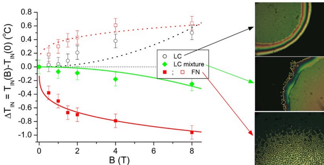
Figure 3. Magnetic field-induced phase transition temperature shifts detected in a calamitic liquid crystal (LC), in its mixture with a bent-core LC, and in a ferronematic (FN) based on them. The lines represent theoretical fits. On the right: microphotographs of the isotropic-to-nematic phase transition in these systems.
