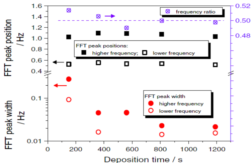
Figure 2. Key parameters of the stability of the electrochemical oscillation.
