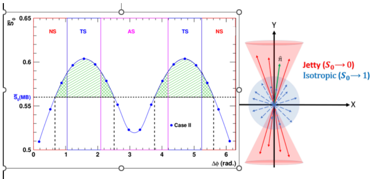
Figure 2: The new extended definition of the CDF-based Underlying Events (TS) in 13 TeV pp collisions in correlation with the sphericity parameter, S_0 in 40% more wider range
