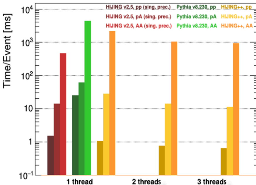
Figure 2. Speedup of the new version of the HIJING++ in comparison to other Monte Carlo simulators.
