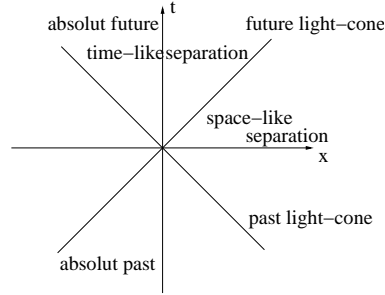
Figure 2.3: The light cones.
