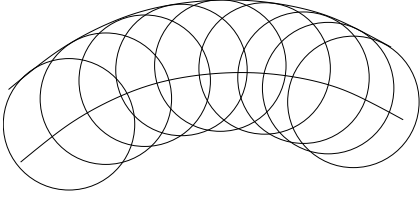
Figure 5.1: Huygens principle for a wave front.
