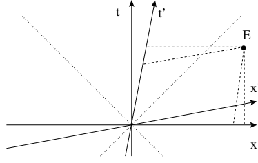
Figure 2.4: Lorentz transformations.
