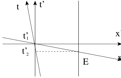
Figure 2.5: Lorentz contraction.
