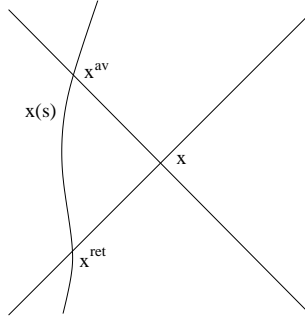
Figure 6.1: The observer at x receives the signal emitted from the point x^{\text{ret}} or x^{\text{av}} for the retarded or the advanced propagation, respectively.
